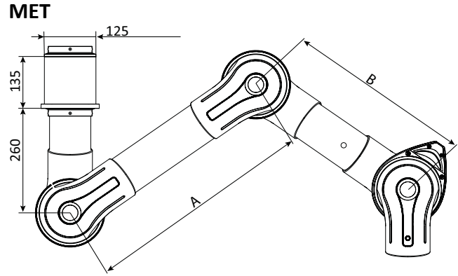
MET for ceiling mounting, excluding ceiling bracket MTI. MEV for wall mounting, including wall bracket MVK.
